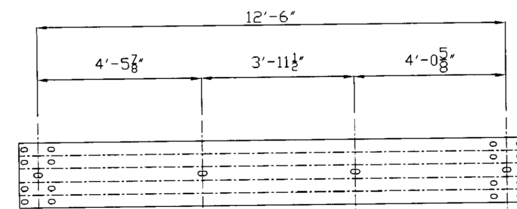
RAIL D - 4 REQ'D
