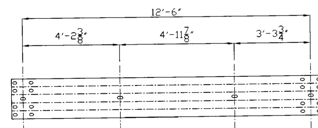
RAIL B - 4 REQ'D
