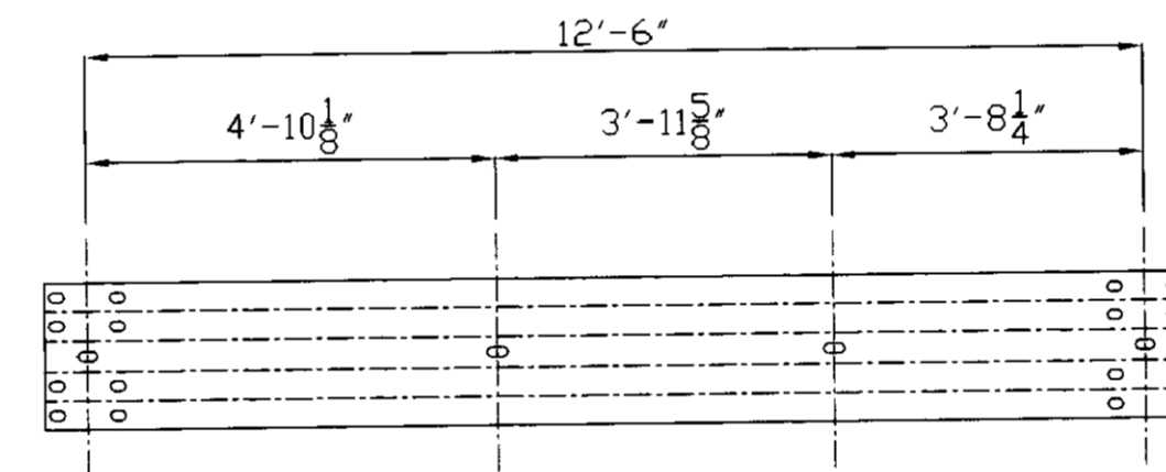
RAIL C - 4 REQ'D
