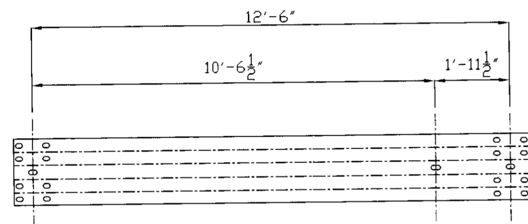
RAIL A - 4 REQ'D
